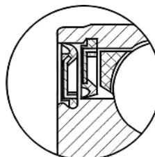
Seal Type B
