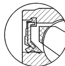
Seal Type C
