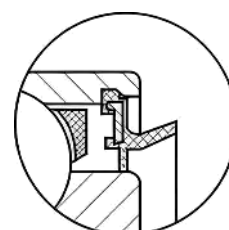
Seal Type S
