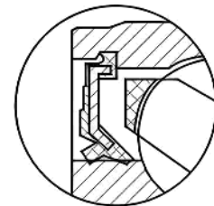
Seal Type C
