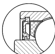
Seal Type A
