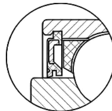
Seal Type A
