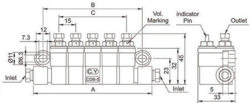
Dimensional Drawing of CDB-5-A-11111-AA
