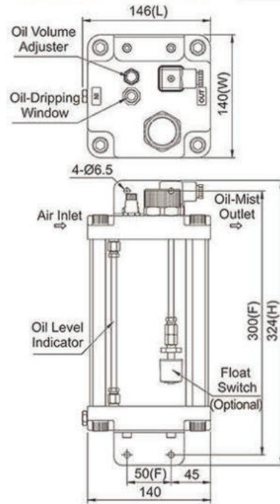
Dimensional Drawing of COM-01-SC
