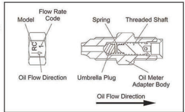
Internal Structure of Oil Meter Adapter
