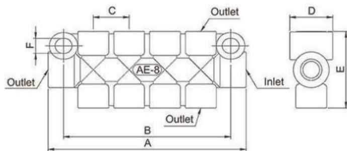
Dimensional Drawing of AE-8-6-4
