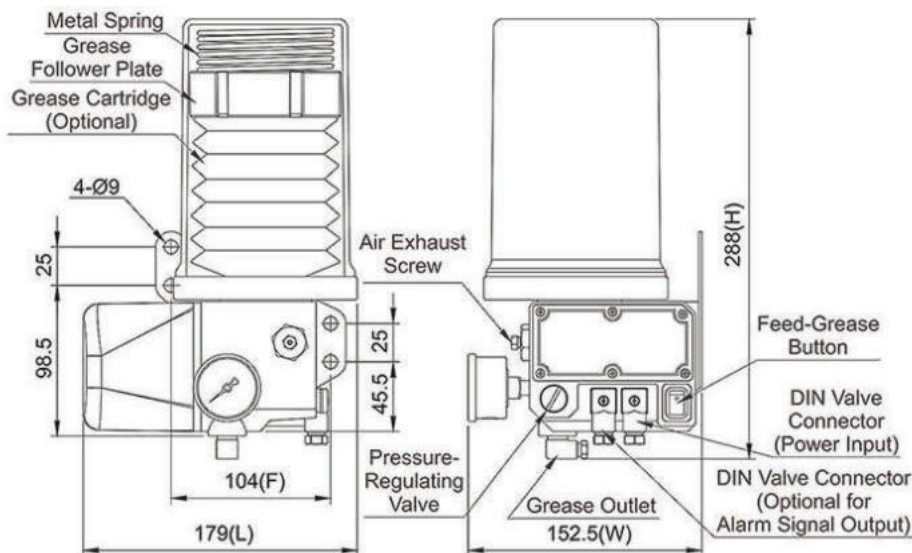
Dimensional Drawing of KACP-07-K-3-PC-RC with Grease Cartridge
