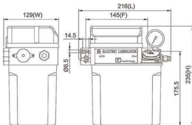
Dimensional Drawing of CEPB-01-C-3-2
