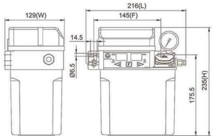
Dimensional Drawing of CESG04-01-2-C-3
