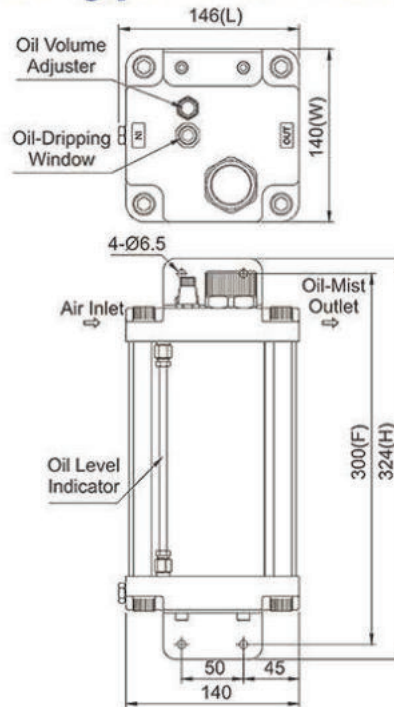
Dimensional Drawing of COM-01
