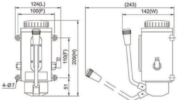
Dimensional Drawing of CLAB-8-R-H-1
