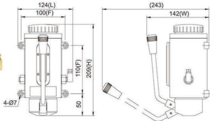
Dimensional Drawing of CLA-8-R-H-1
