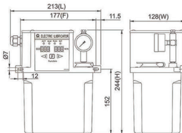
Dimensional Drawing of CEN04-01-2-C-3
