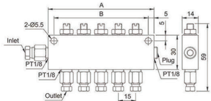
Dimensional Drawing of CB-5-6-4
