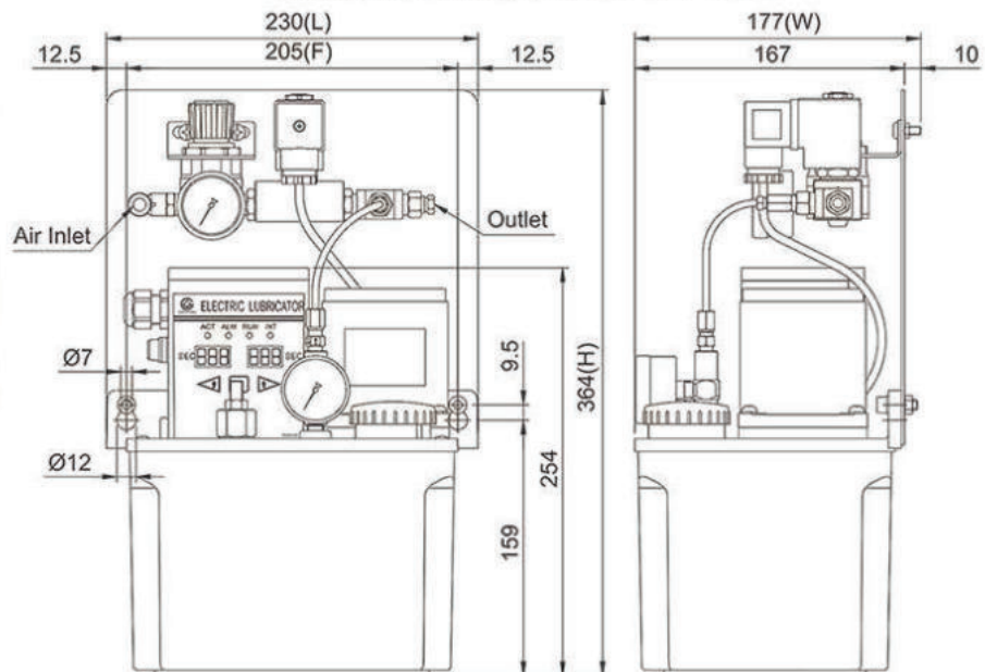
Dimensional Drawing of CEN23-03-1-C-25-3
