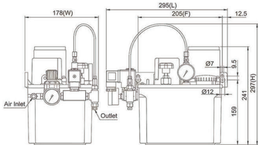
Dimensional Drawing of CEN24-03-C-25-3
