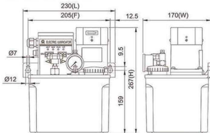
Dimensional Drawing of KGNV-03-C-40-3
