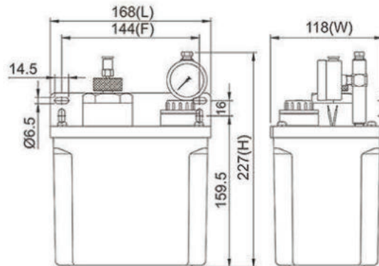
Dimensional Drawing of PNA-01-3-0
