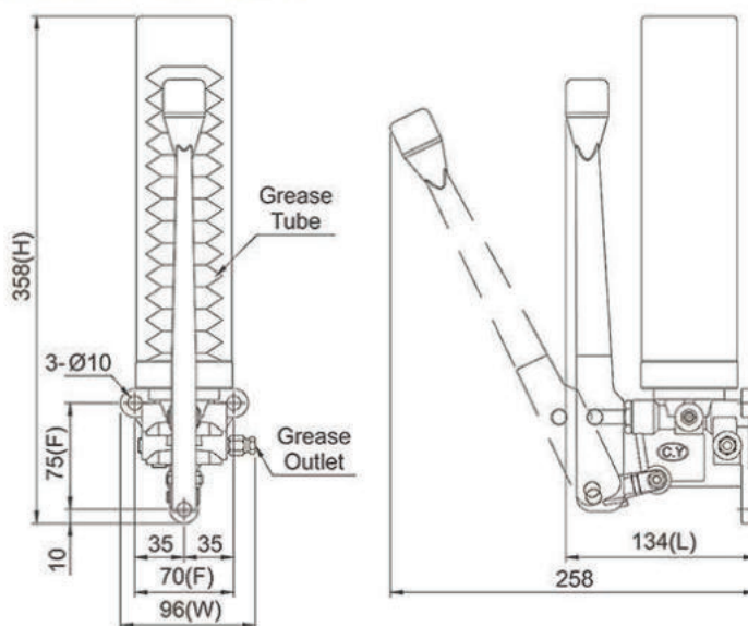
Dimensional Drawing of CLHA-25-R-D-1-A with Grease Tube
