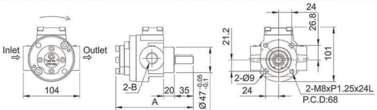
Dimensional Drawing of Heavy Oil Pump
