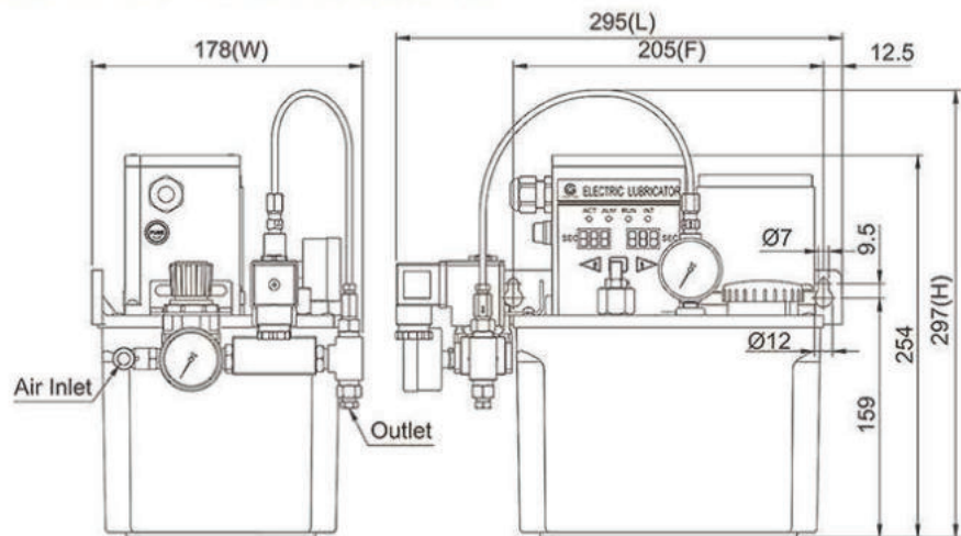
Dimensional Drawing of CEN22-03-1-C-25-3
