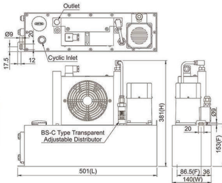
Dimensional Drawing of CLSS-08-M-90-A-A
