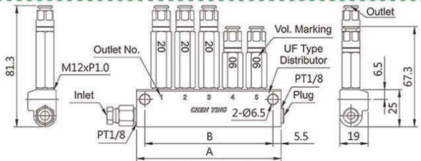
Dimensional Drawing of CFB-05-B-55522-AG
