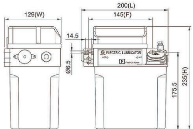
Dimensional Drawing of CESP-01-C-1-2
