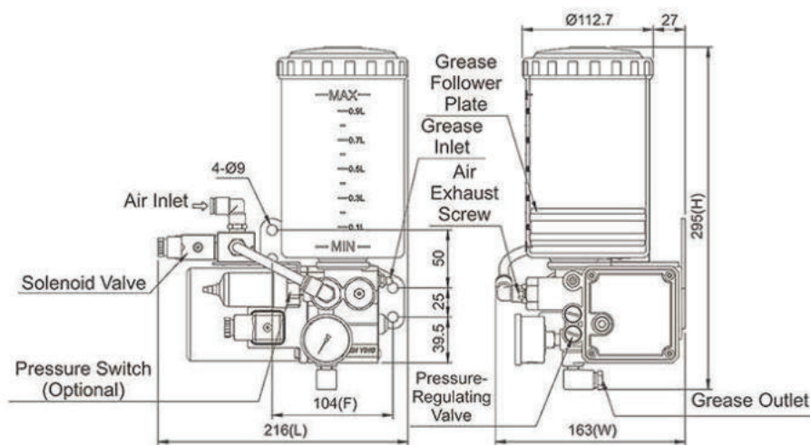
Dimensional Drawing of KGB-35-C-5-PC
