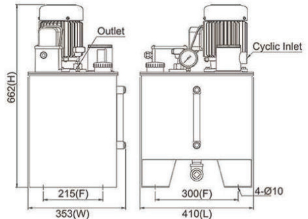
Dimensional Drawing of CLS-10-36-D-2-3-C
