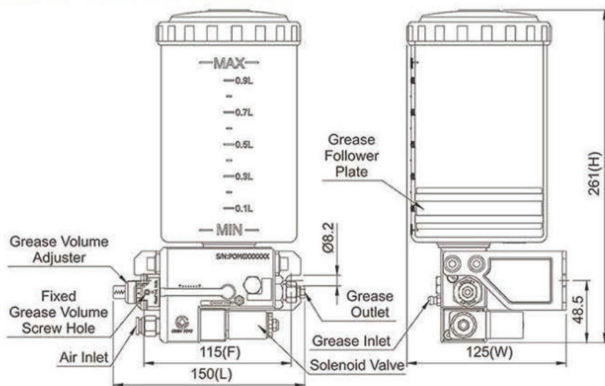
Dimensional Drawing of POM-A-35-1-K-0
