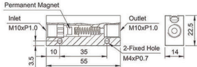
Standard Type Magnetic Sensor Reed Switch
