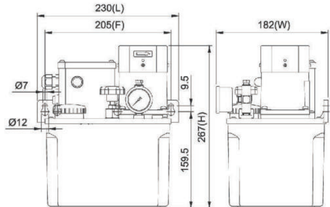
Dimensional Drawing of KGV-03-C-40-3
