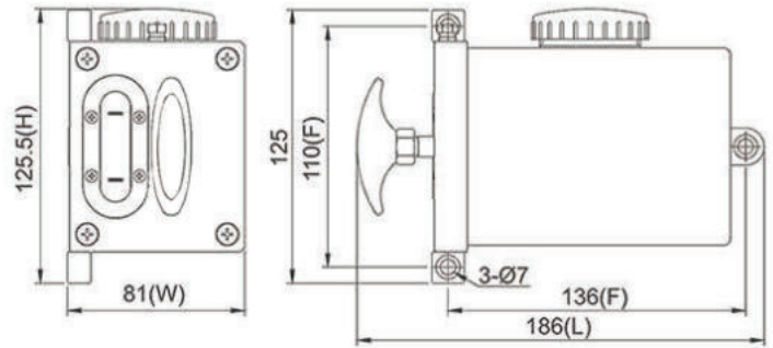
Dimensional Drawing of CTA-8-R-U-0
