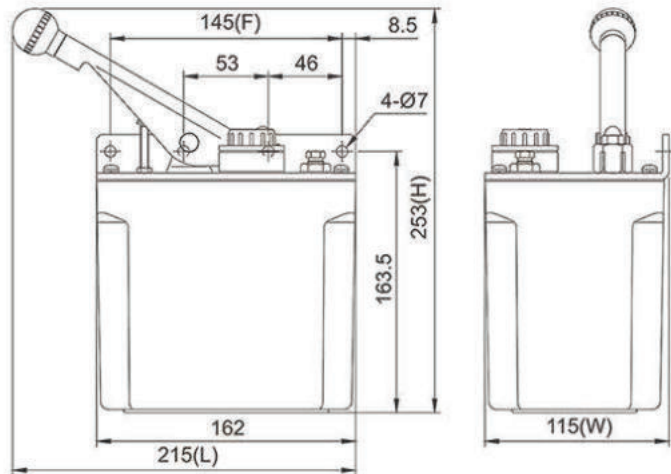
Dimensional Drawing of CKE-20-R-0
