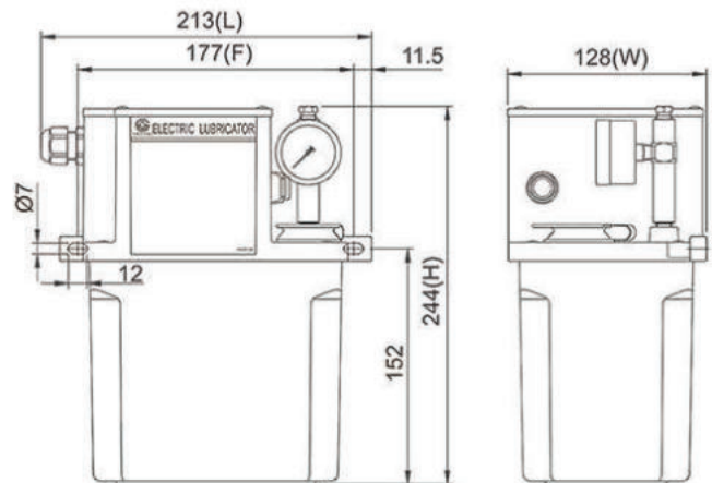
Dimensional Drawing of CEN01-01-C-3
