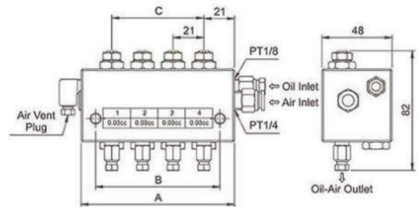
Dimensional Drawing of OC-4-A-2222
