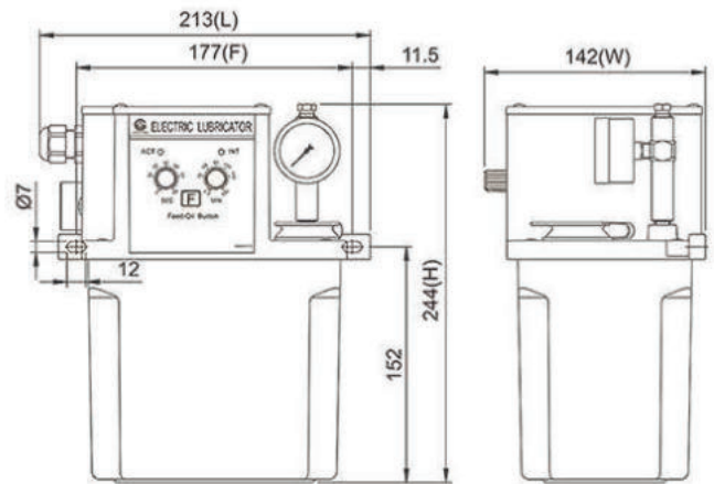
Dimensional Drawing of CEWB-01-2-C-3-2
