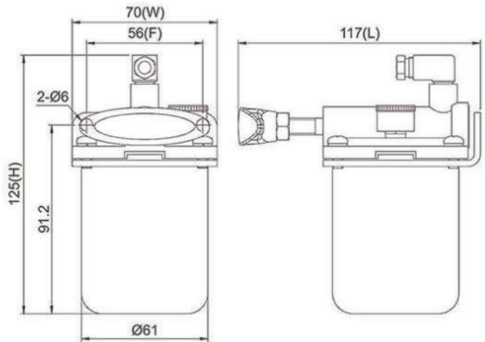
Dimensional Drawing of CTA-3-H-0
