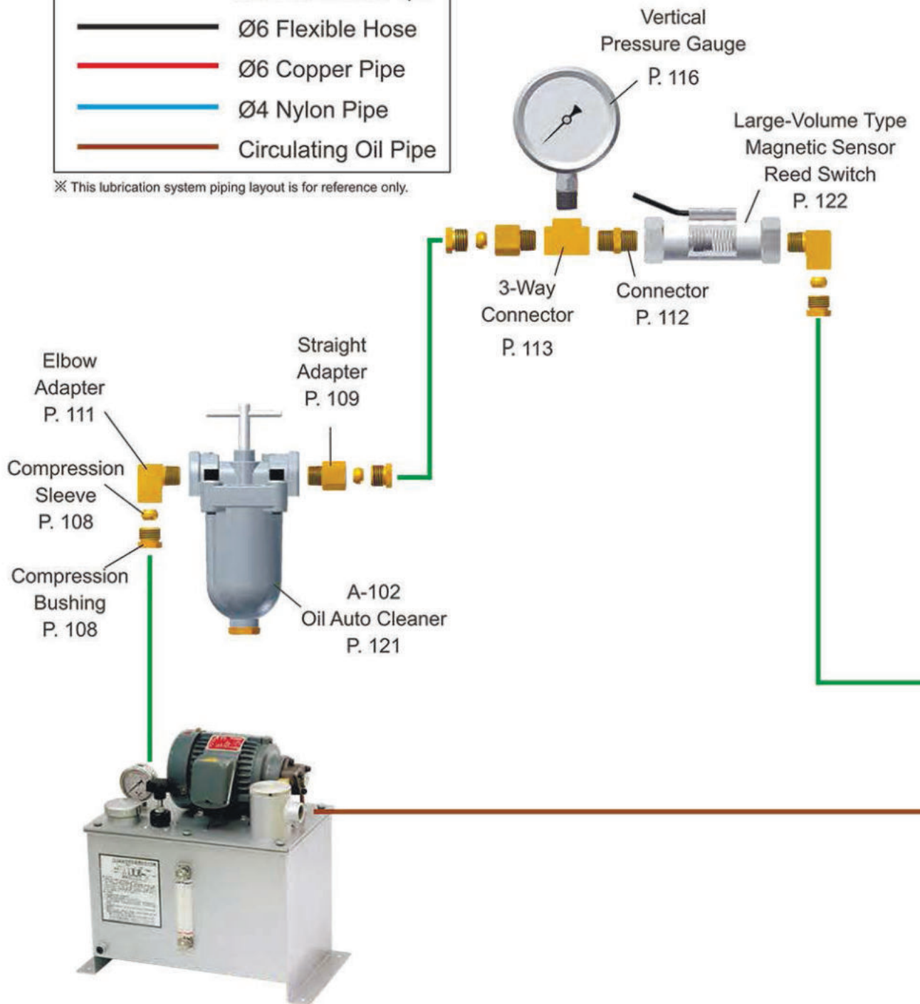
CLSB Circulating Type Oil Electric Lubricator P. 23
