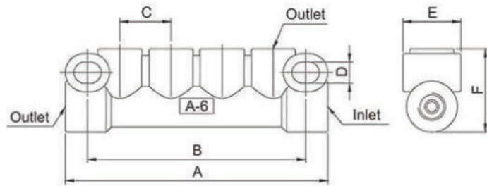
Dimensional Drawing of A-6-6-4
