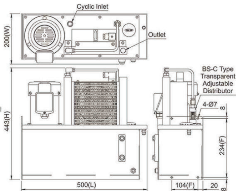
Dimensional Drawing of CLSS-14-13-1-D-A-A
