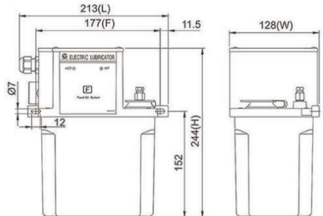
Dimensional Drawing of CESD-01-2-C-1-2
