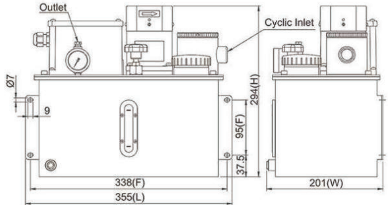
Dimensional Drawing of CEU-08-C-25-3-A
