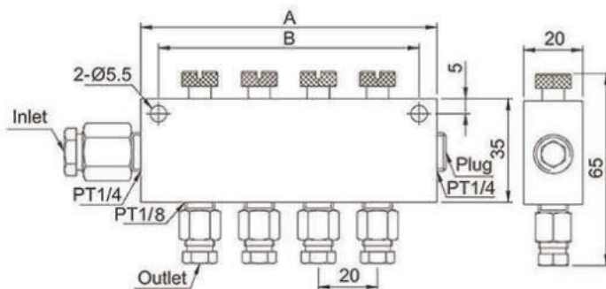
Dimensional Drawing of AB-4-8-6
