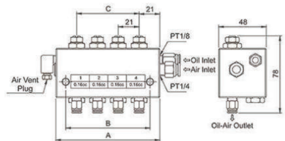
Dimensional Drawing of OC-4-B-5555
