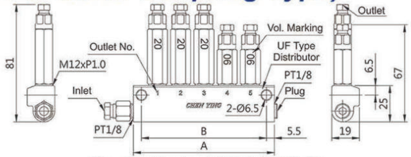
Dimensional Drawing of CFB-05-A-55522-AG
