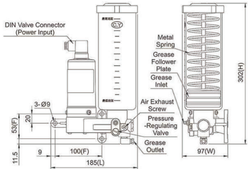
Dimensional Drawing of KGAP-40-K-1
