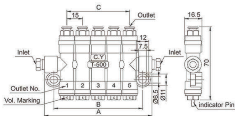
Dimensional Drawing of T-500-B-33333-AA
