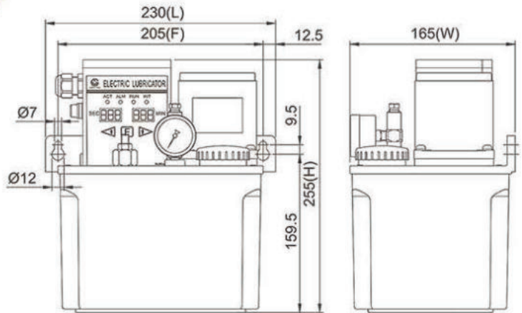
Dimensional Drawing of CENA-03-2-C-25-3
