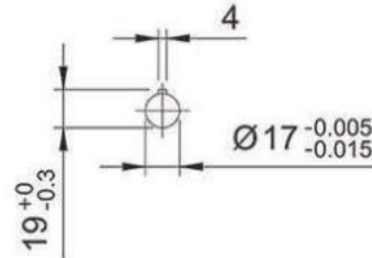
Shaft Size of CYP-216, 220
