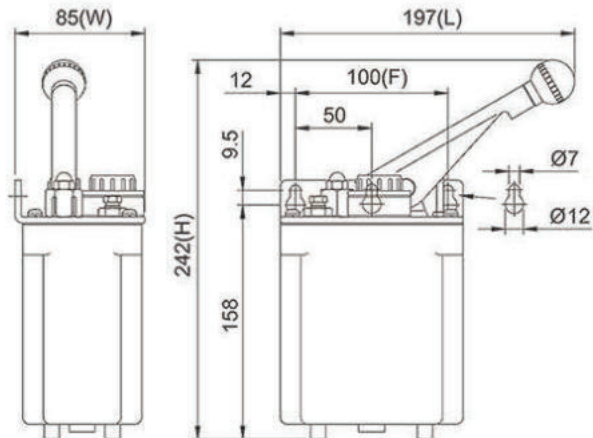
Dimensional Drawing of CKE-8-L-0
