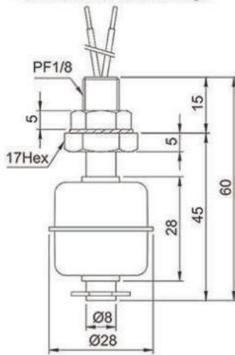
M21004 Galvanized Iron Float Ball
