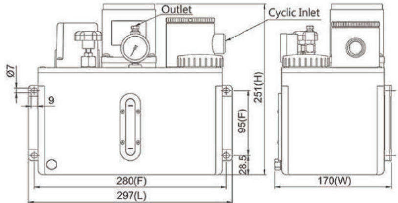
Dimensional Drawing of CEH-05-C-25-3-A
