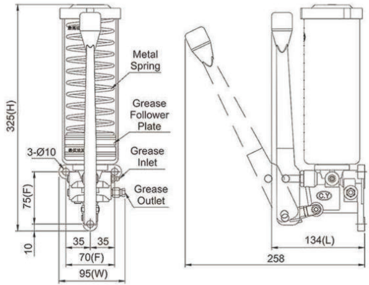
Dimensional Drawing of CLHP-40-R-D-1
