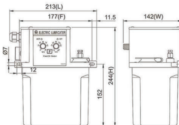
Dimensional Drawing of CESW-01-2-C-1-2
