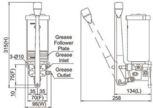
Dimensional Drawing of CLHA-20-R-D-1
