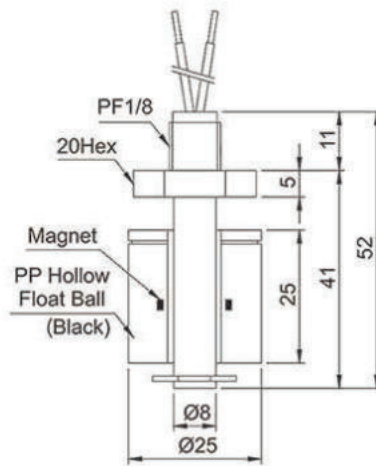
M21002 Black Float Ball
