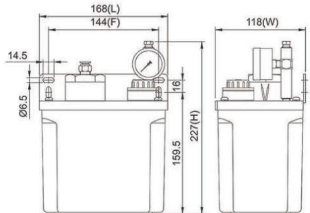
Dimensional Drawing of PNB-01-3-0
