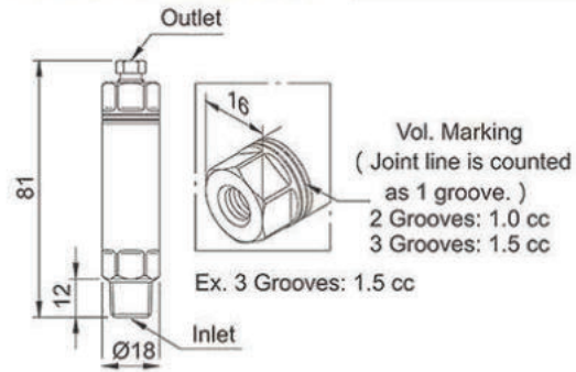
Dimensional Drawing of CCB-1-A-6
