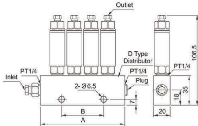
Dimensional Drawing of CCB-4-6666-AG
