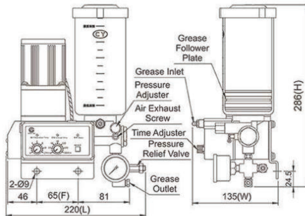
Dimensional Drawing of KSB-30-180-C-3
