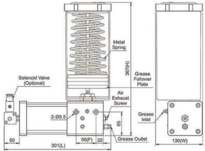
Dimensional Drawing of MAG-50-0-1-A
