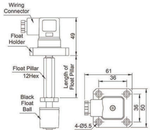
M21002 Black Float Ball W/Float Pillar, Float Holder, and Wiring Connector
