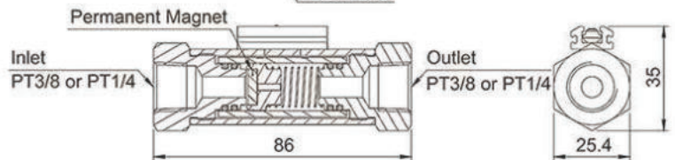
Large-Volume Type Magnetic Sensor Reed Switch
