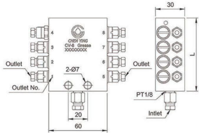
Dimensional Drawing of CV-8-6-4-1
